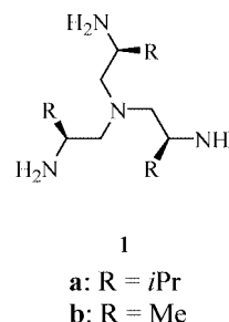
Figure 1. Chiral TREN compounds.
