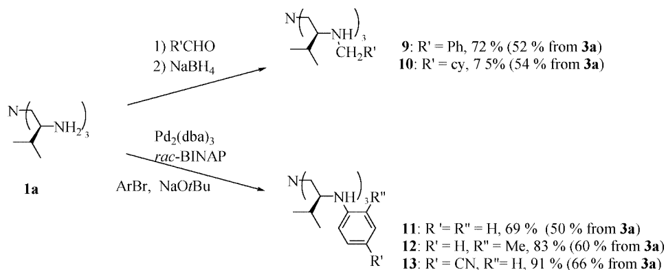
Scheme 4. N -Functionalization of chiral TREN.
