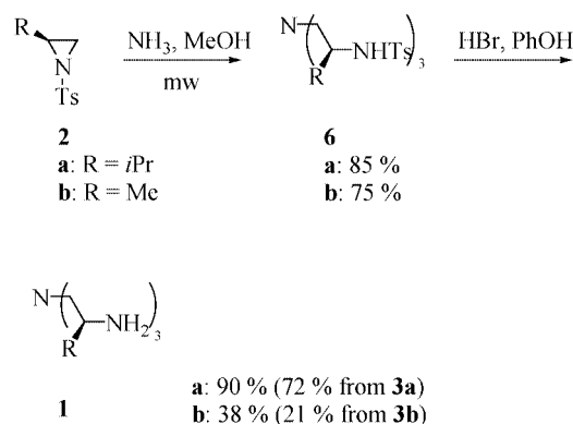
Scheme 2. Synthesis of chiral TREN derivatives by aziridine ring opening.
