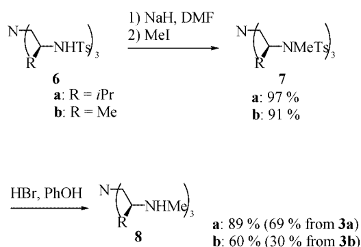
Scheme 3. Synthesis of chiral N -alkylated TREN derivatives.
