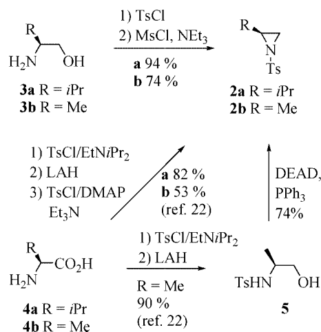
Scheme 1. Synthesis of chiral tosylaziridines.
